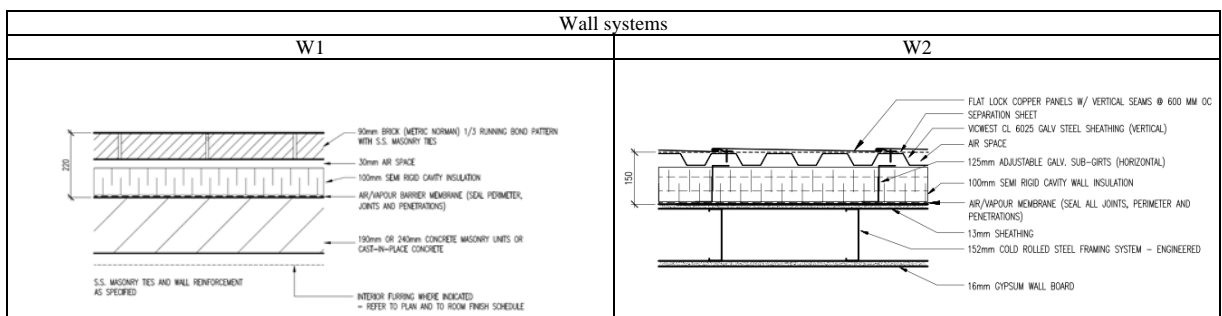
Fig. 2. Wall system components (base case), reference: Diamond Schmitt Architects.
